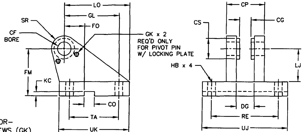
DIMENSIONS IN MILLIMETERS
